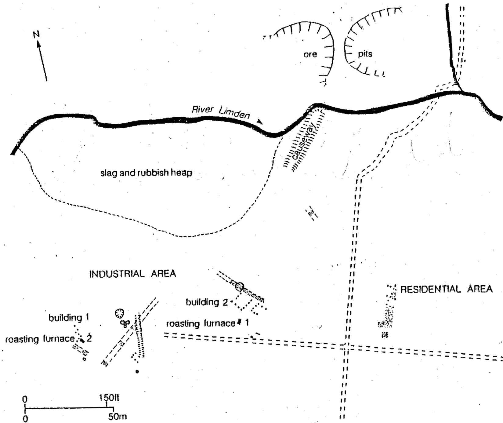
Fig.23 Layout of Roman ironmaking settlement at Bardown.
